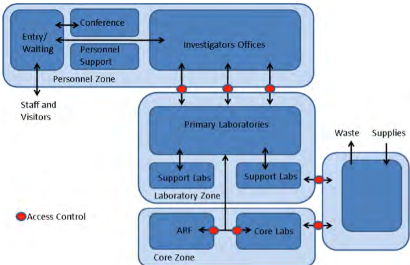
Figure 2.1.3.3 Relational diagram. Typical functional relationships and adjacencies ARF = Animal research facility
