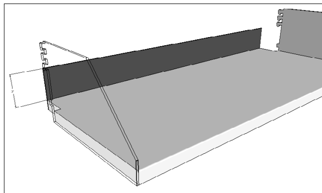
Figure 4.5.3 Typical Lab Shelf & Flanges
