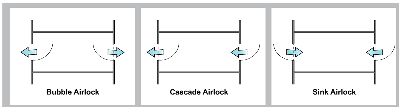
Figure 13.1.3 Airlock Configurations
