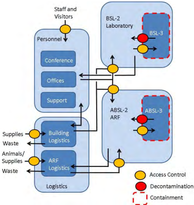
Figure 2.5.3.3(B) Example of relationships between primary building zones, including containment zones
