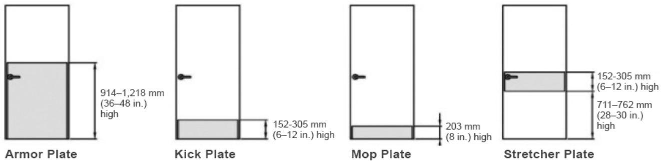
Figure 4.2.1.6 Door Plate Types
