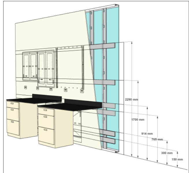
Figure 4.3.2.1 Wall Strapping
