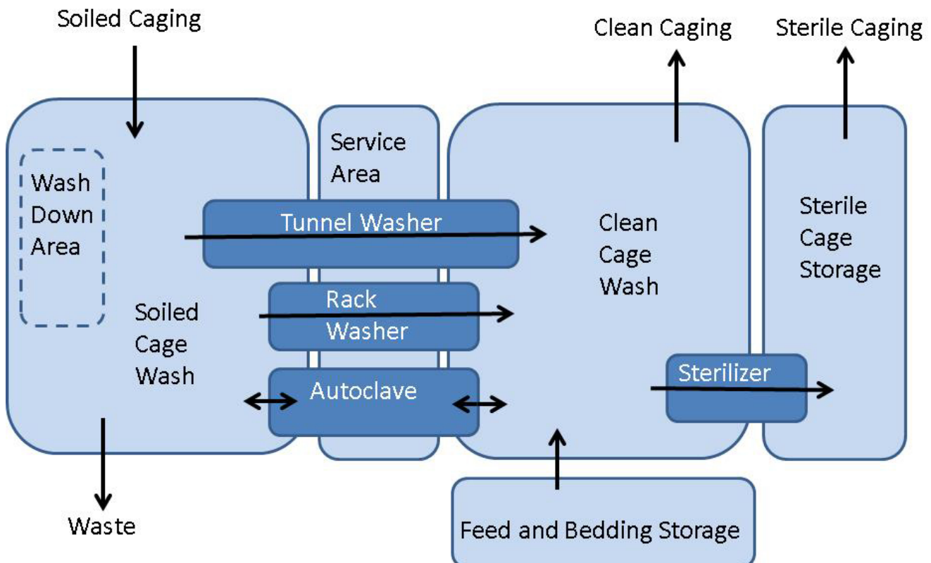
Figure 2.3.4.2 Typical cage wash area relational diagram
