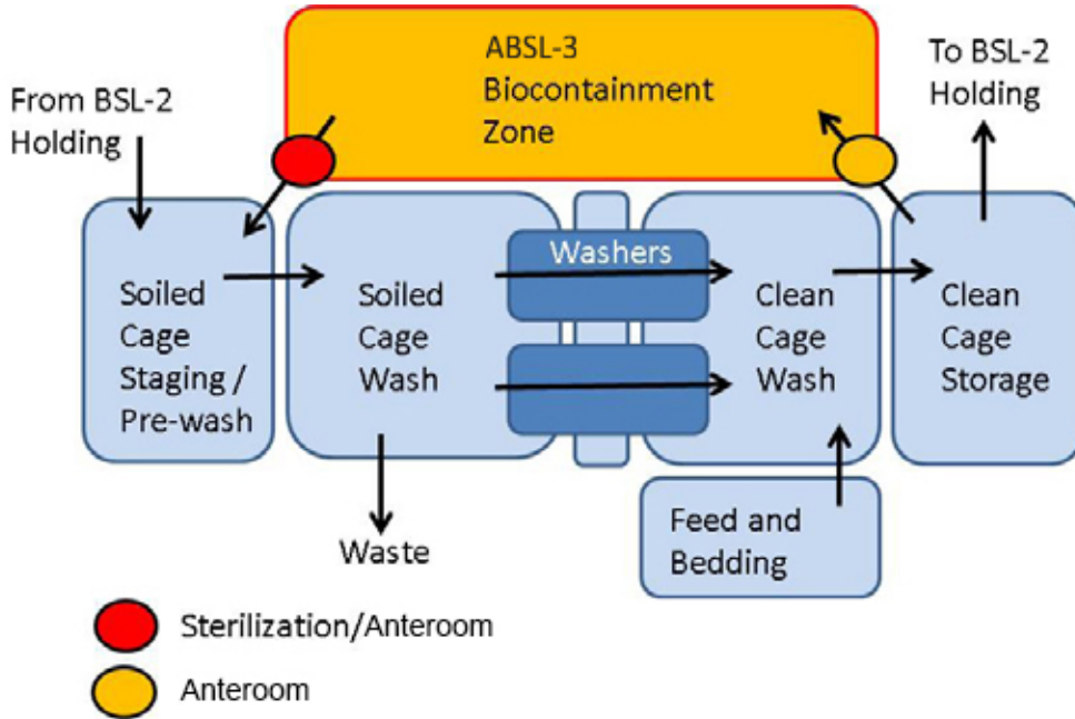
Figure 2.5.3.3(A) Typical relationships between cage processing functions and ABSL-3 zone
