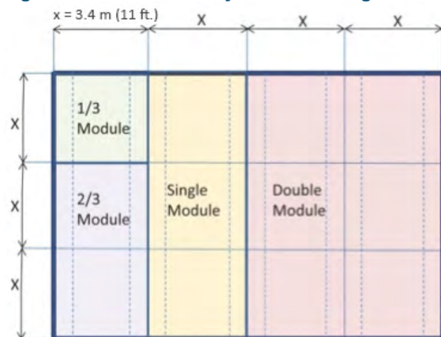
Figure 2.2.2.1 Laboratory module configuration
