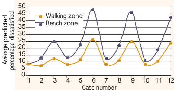
FIGURE 3. Average PPD in walking and bench zones.
