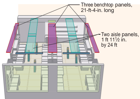
FIGURE 5. Two sets of ceiling-mounted cooling panels.
