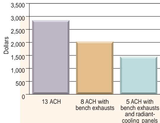
FIGURE 7. Annual cooling costs for three cases.
