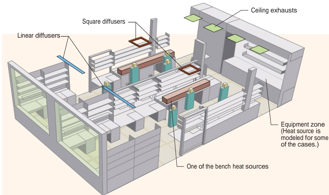
FIGURE 1. Baseline laboratory-model layout.
