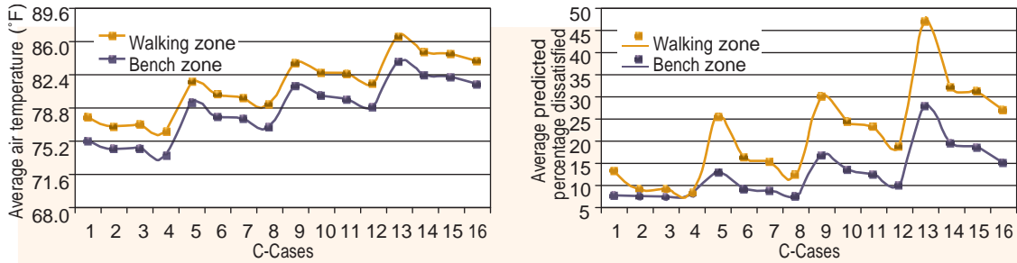
FIGURE 6. Average air temperature and PPD in occupied zones.
