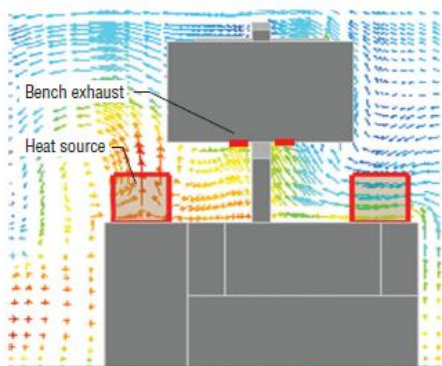
FIGURE 4. Velocity vector at a vertical plane parallel to a window wall.
