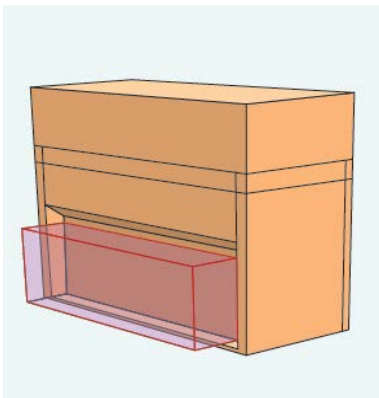
FIGURE 5. The fume hood and the contaminant leak in front of the sash opening.
