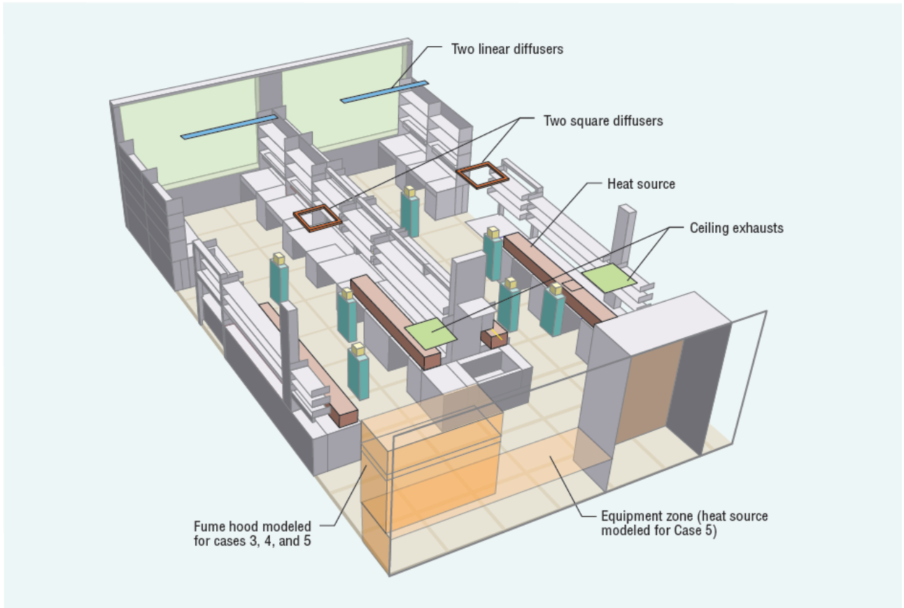
FIGURE 1. Baseline laboratory-model layout.
