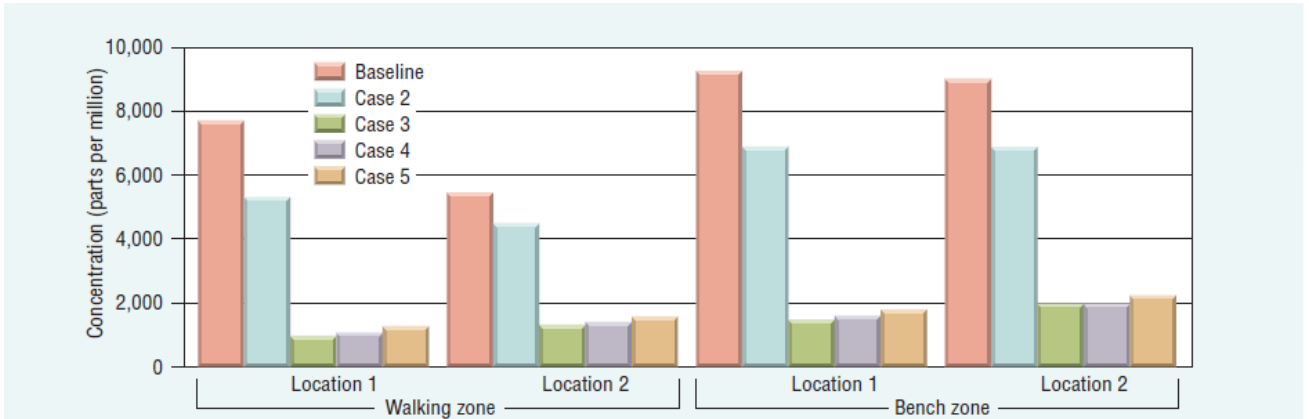
FIGURE 8. Average contaminant concentration levels in the walking and bench zones with the four spill locations.
