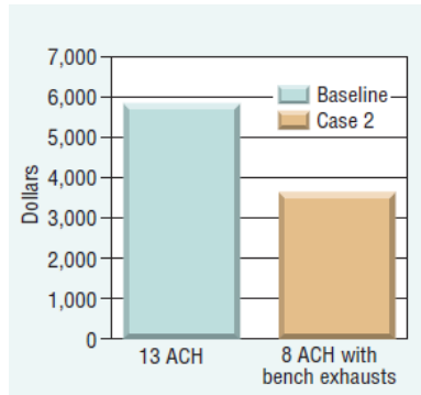
FIGURE 9. Annual HVAC operating costs for a typical laboratory in Washington, D.C. rate.
