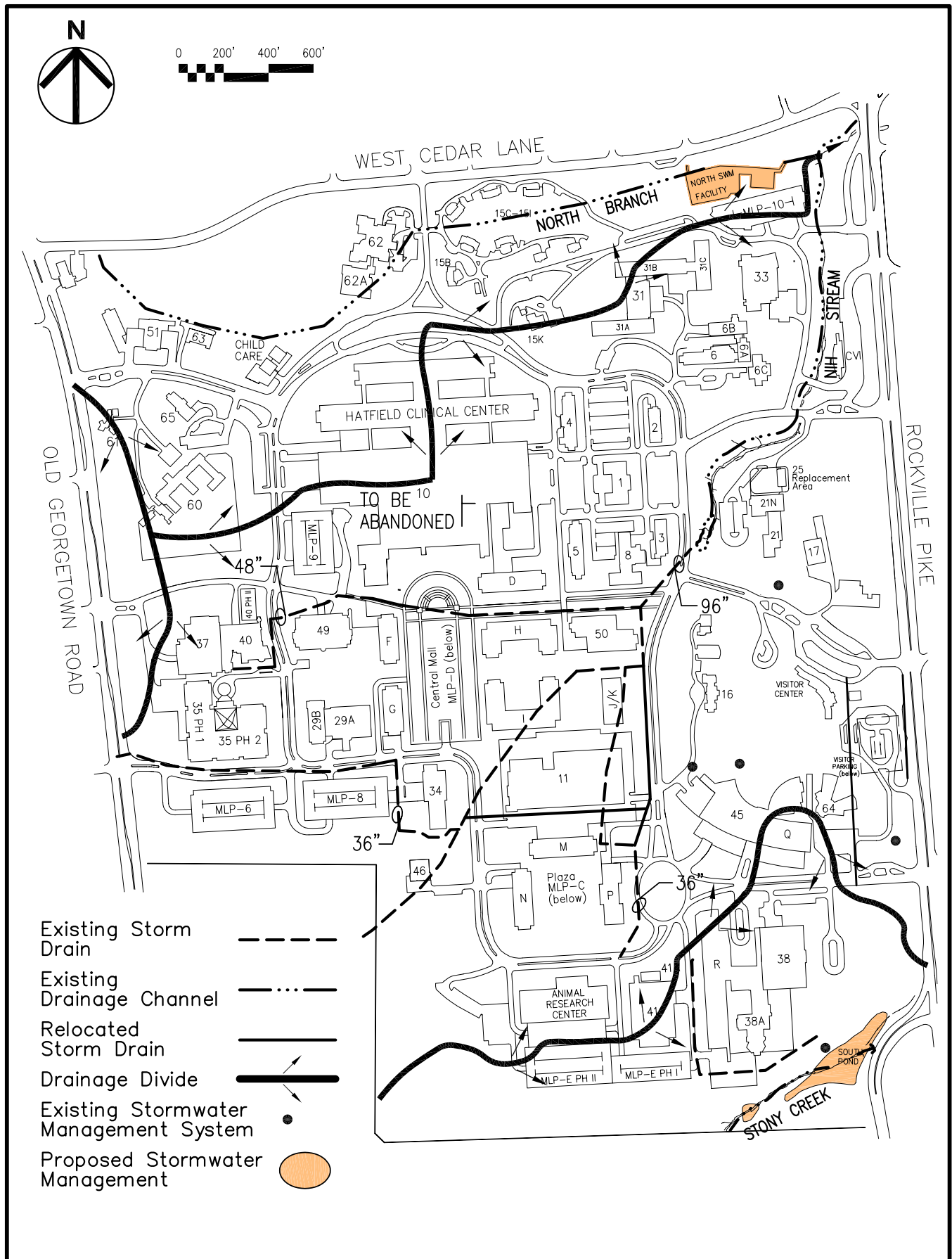
FIGURE 5-17 NIH STORMWATER DRAINAGE.
