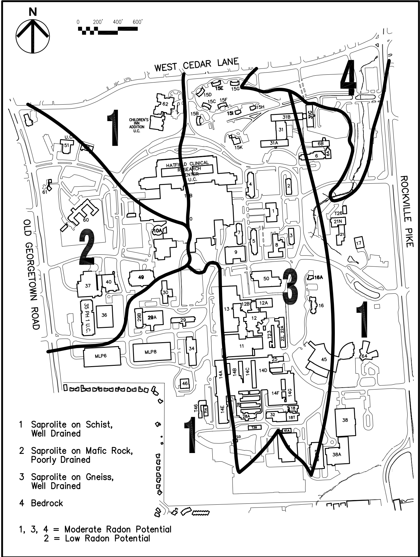
FIGURE 5-25 SUBSURFACE SOILS.
