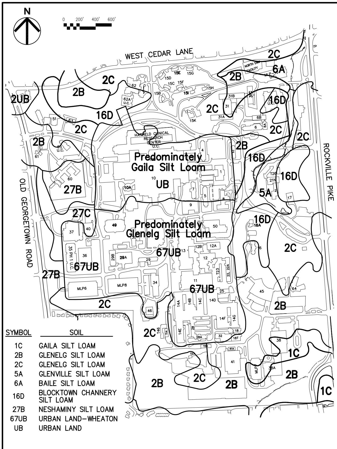
FIGURE 5-26 SURFACE SOILS.
