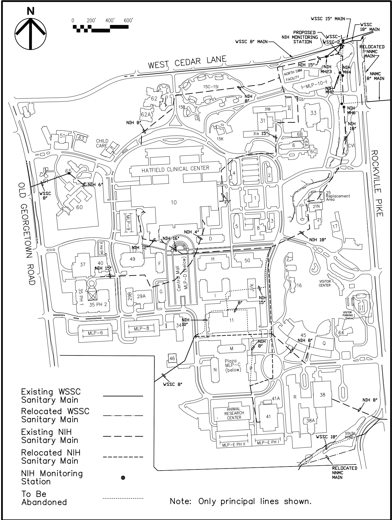
FIGURE 5-16 SANITARY SEWER MAINS.
