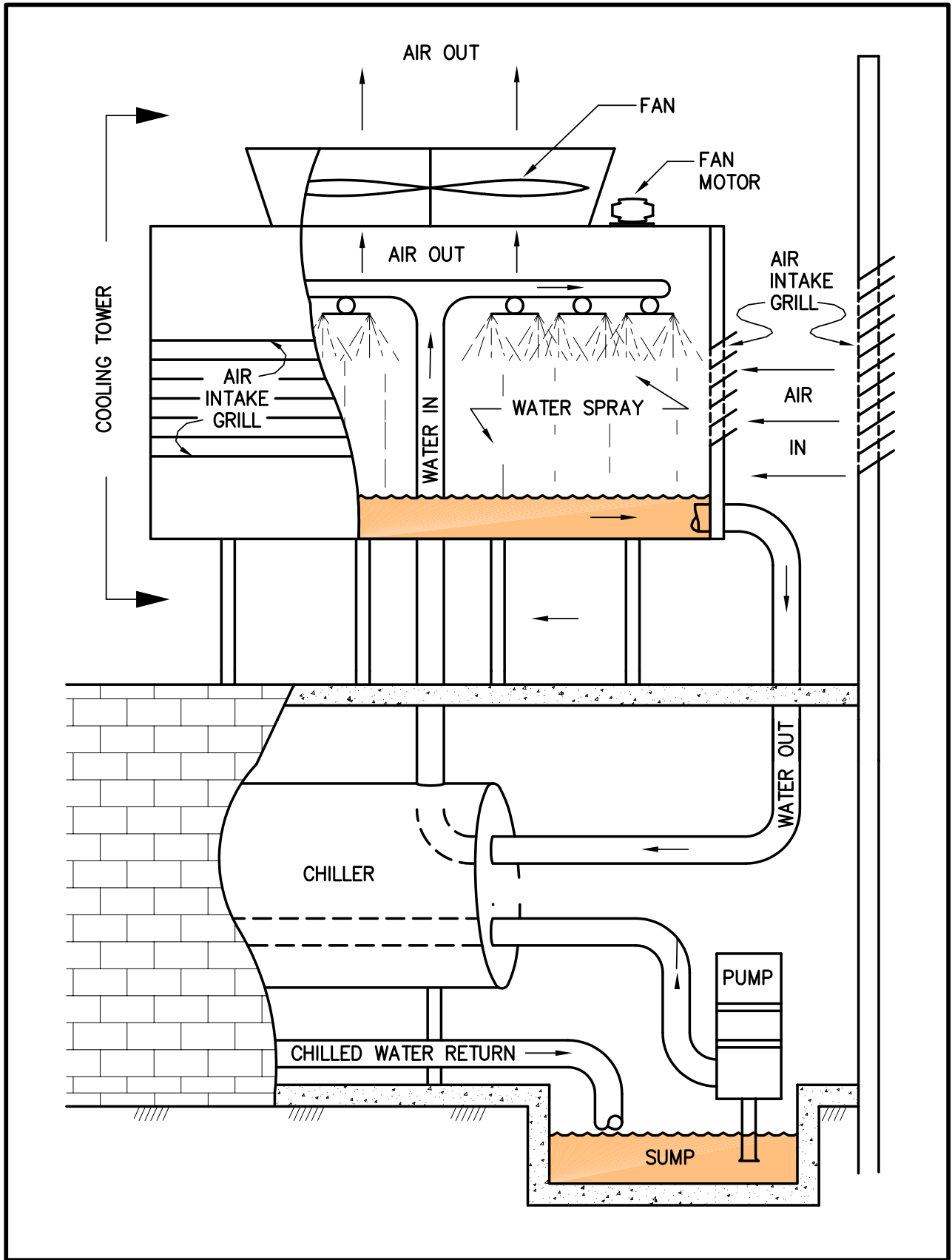
FIGURE 5-19 REFRIGERATION PLANT SCHEMATIC.
