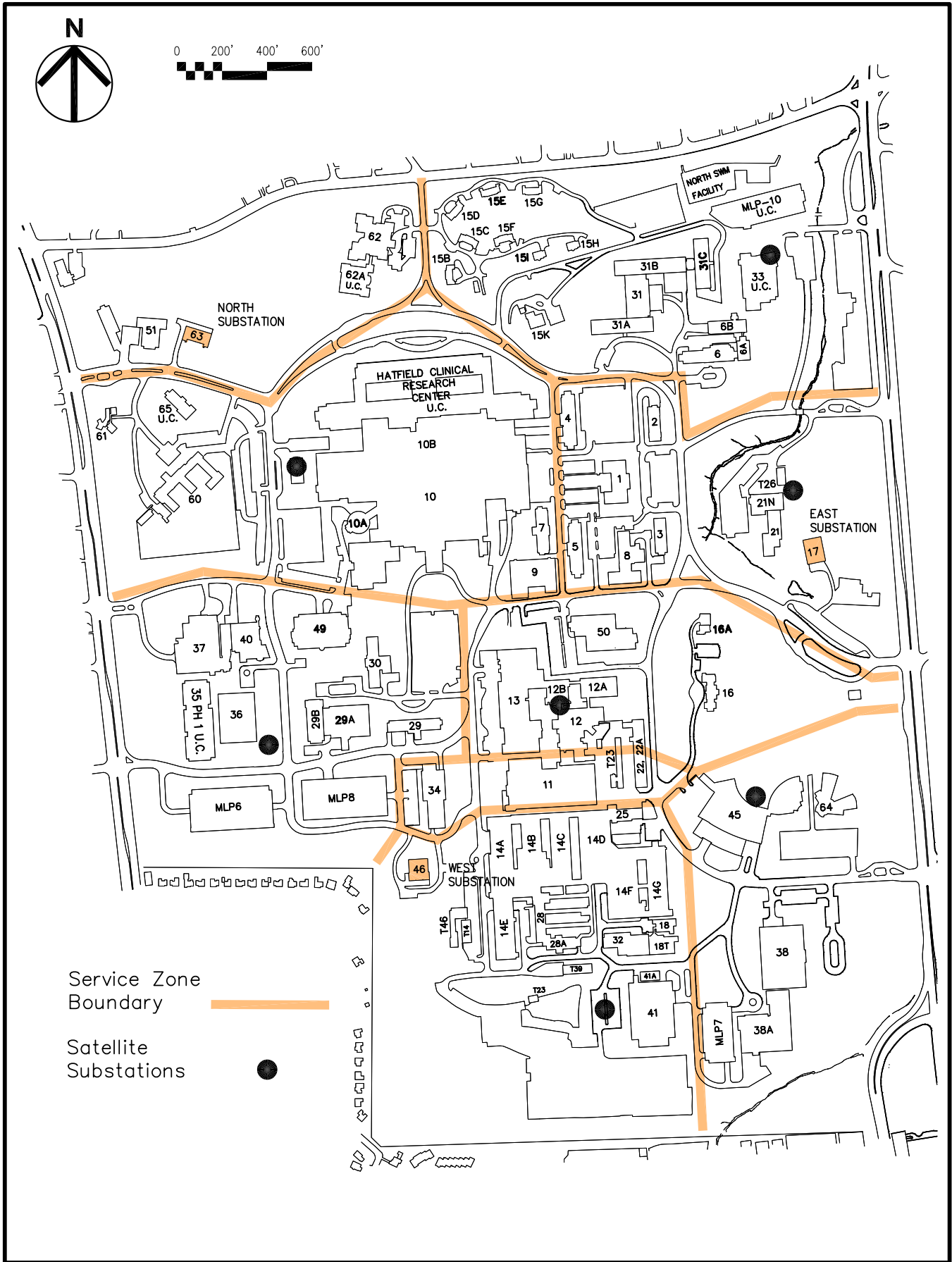
FIGURE 5-14 NIH ELECTRIC POWER SERVICE ZONES AND SUBSTATIONS.
