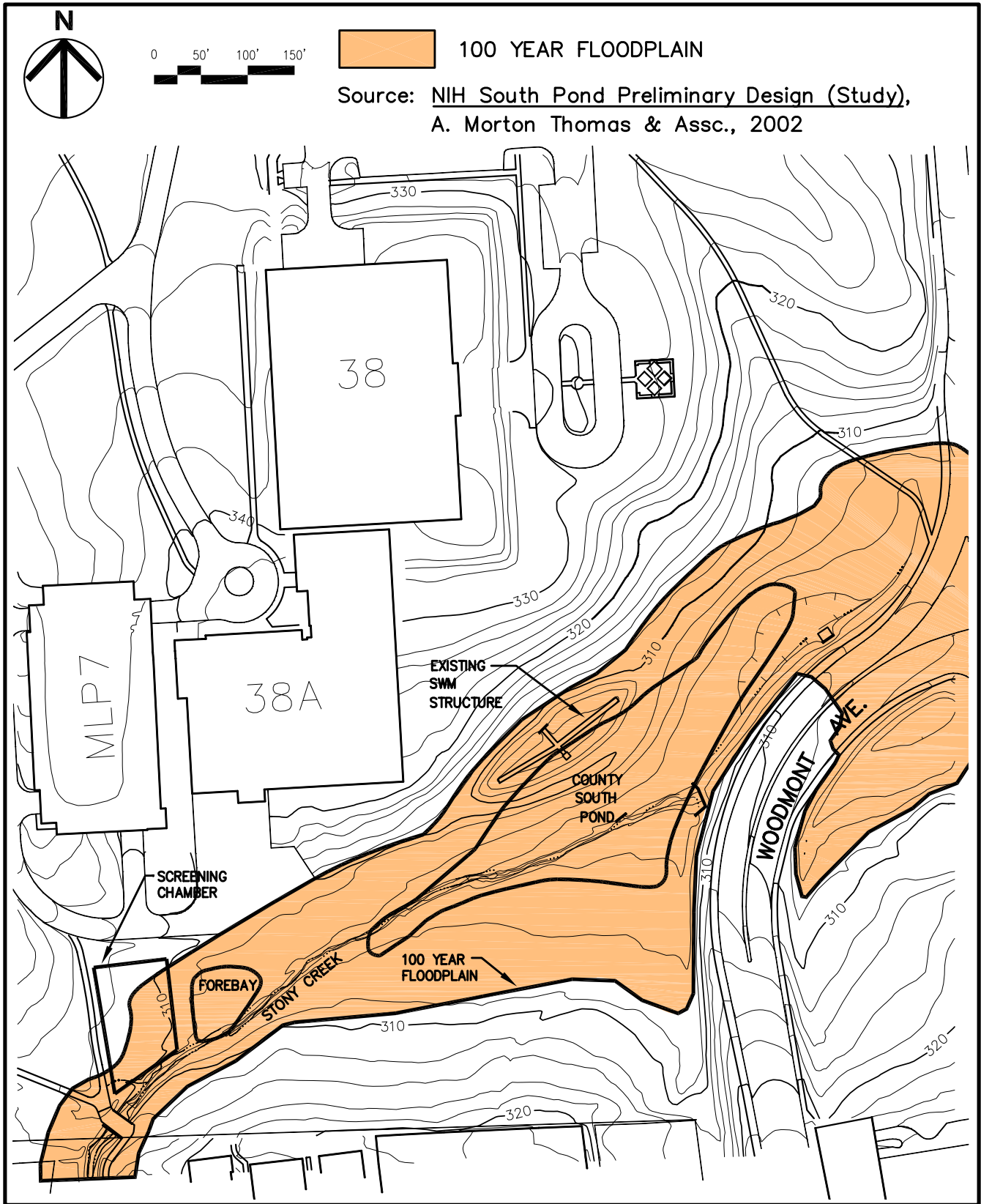
FIGURE 5-29 STONY CREEK 100 YEAR FLOODPLAIN AND SOUTH POND.
