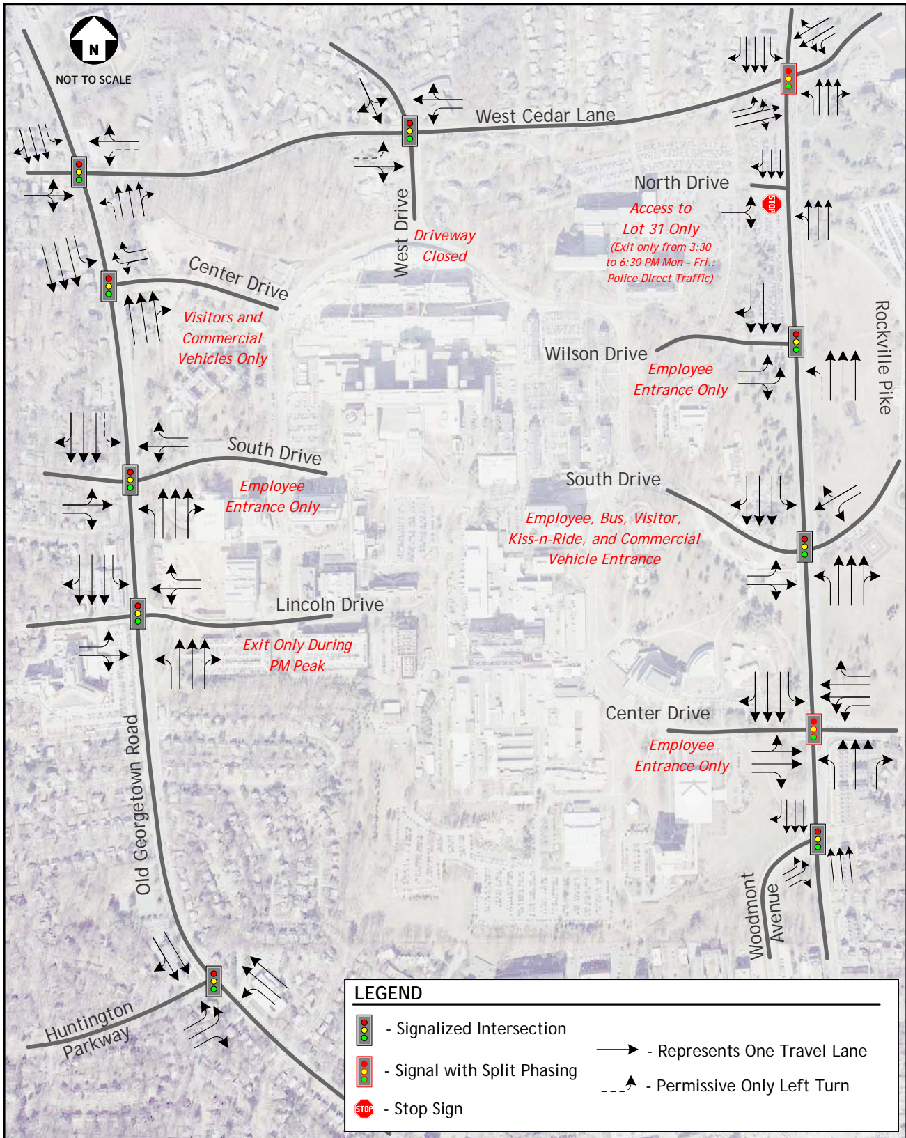
FIGURE G-2 EXISTING LANE CONFIGURATION AND TRAFFIC CONTROL DEVICES.
