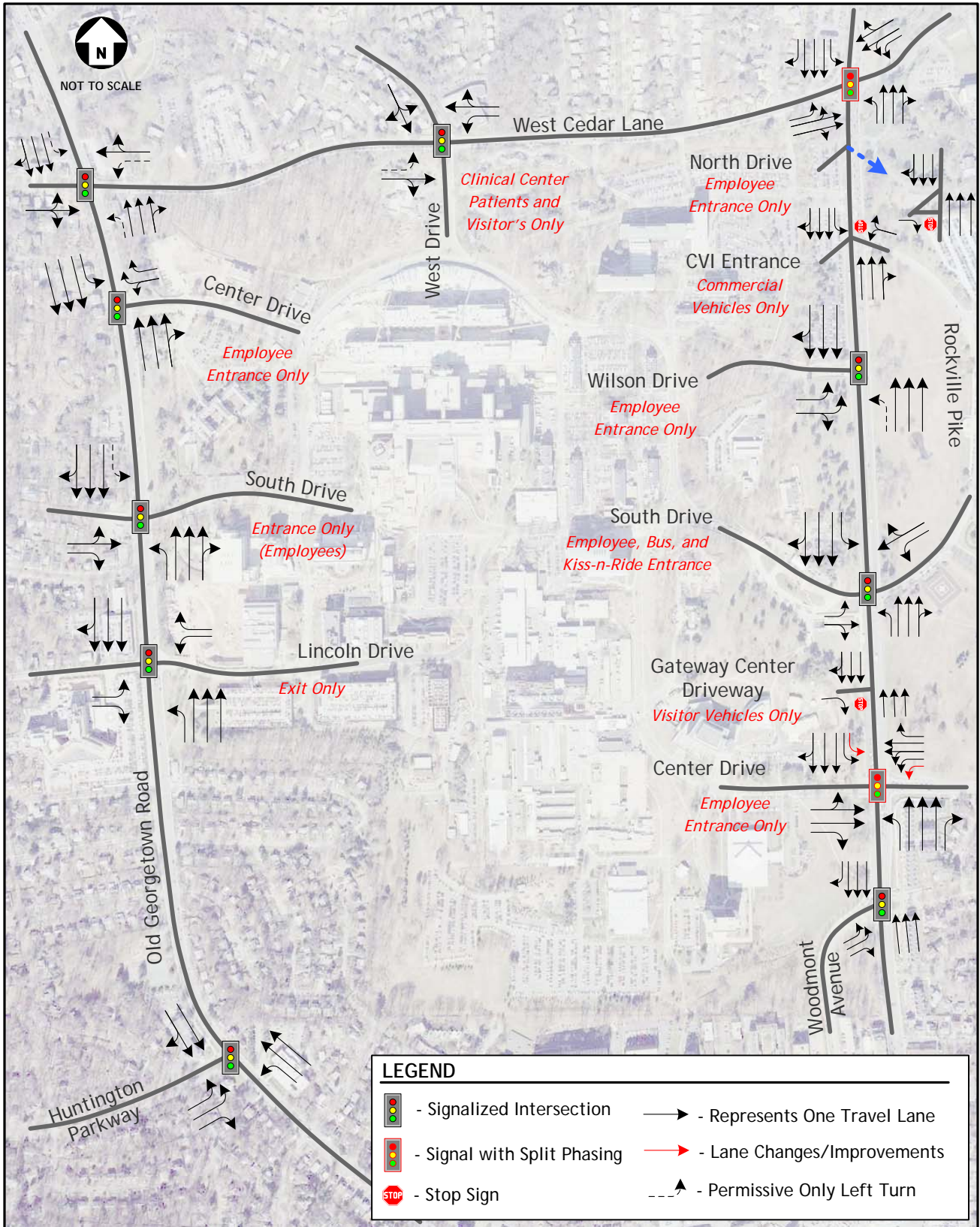
FIGURE G-7 FUTURE LANE CONFIGURATION AND TRAFFIC CONTROL DEVICES.
